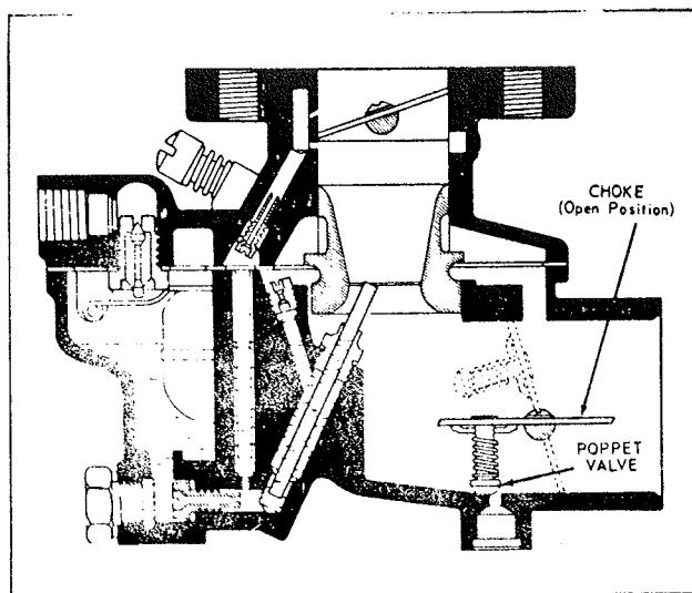
Fig. 5. Choke System
