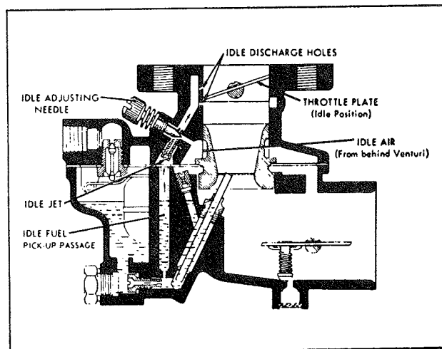
Fig. 3. Idle System
