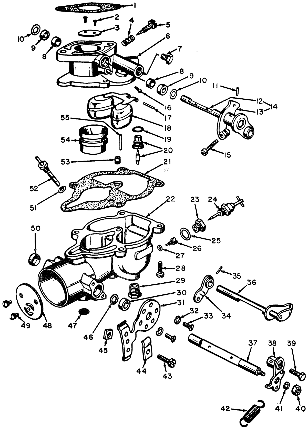
Fig. 6. Exploded View
