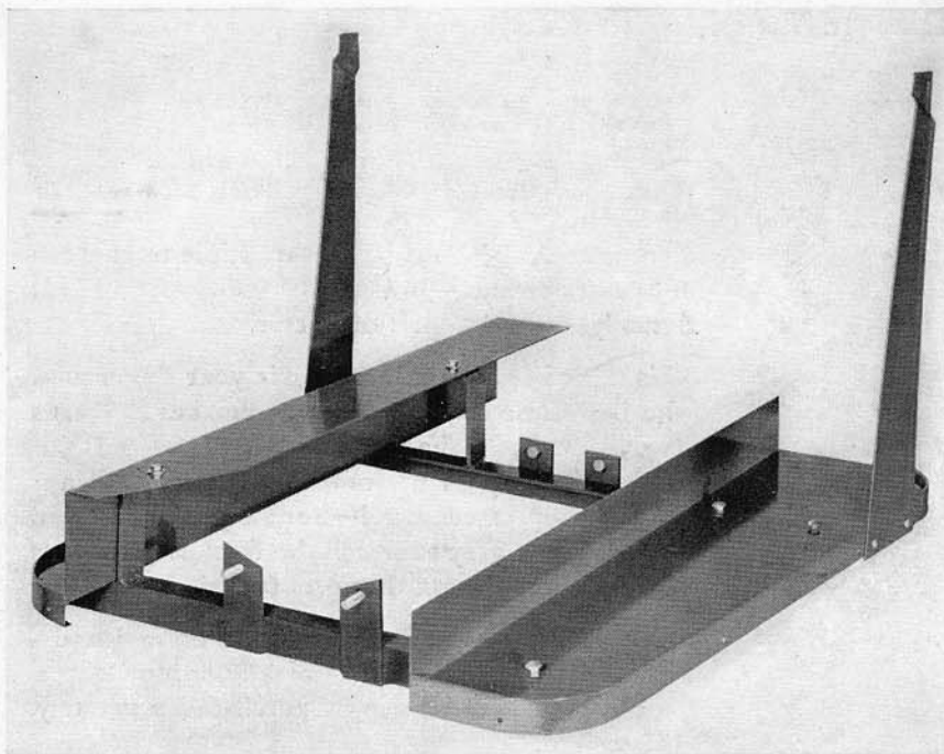
(Running Boards Assembled Showing Rear Wheel Guards)
